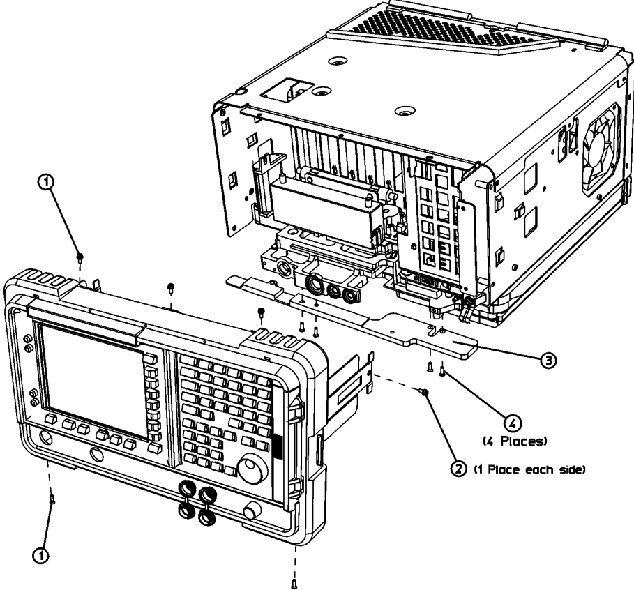
Figure 15 Front Frame Assembly Replacement
