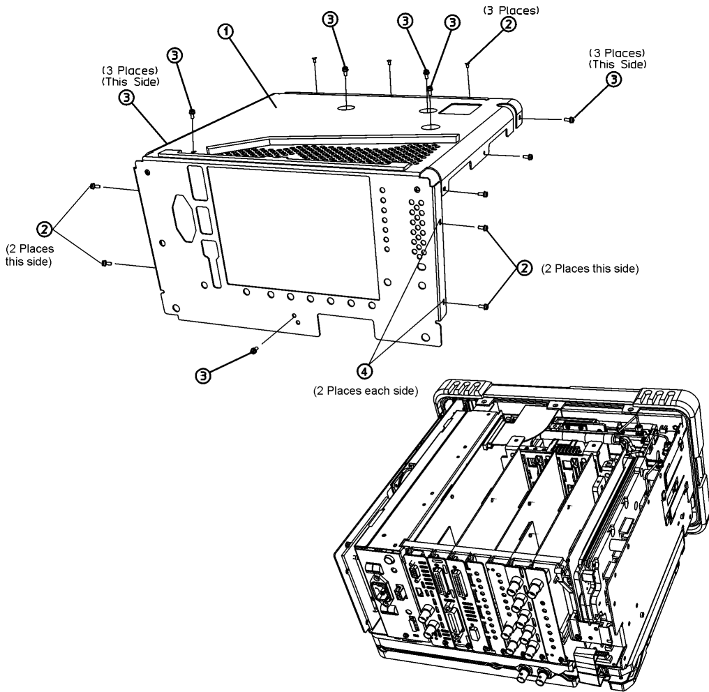
Figure 17 Chassis Cover Replacement
