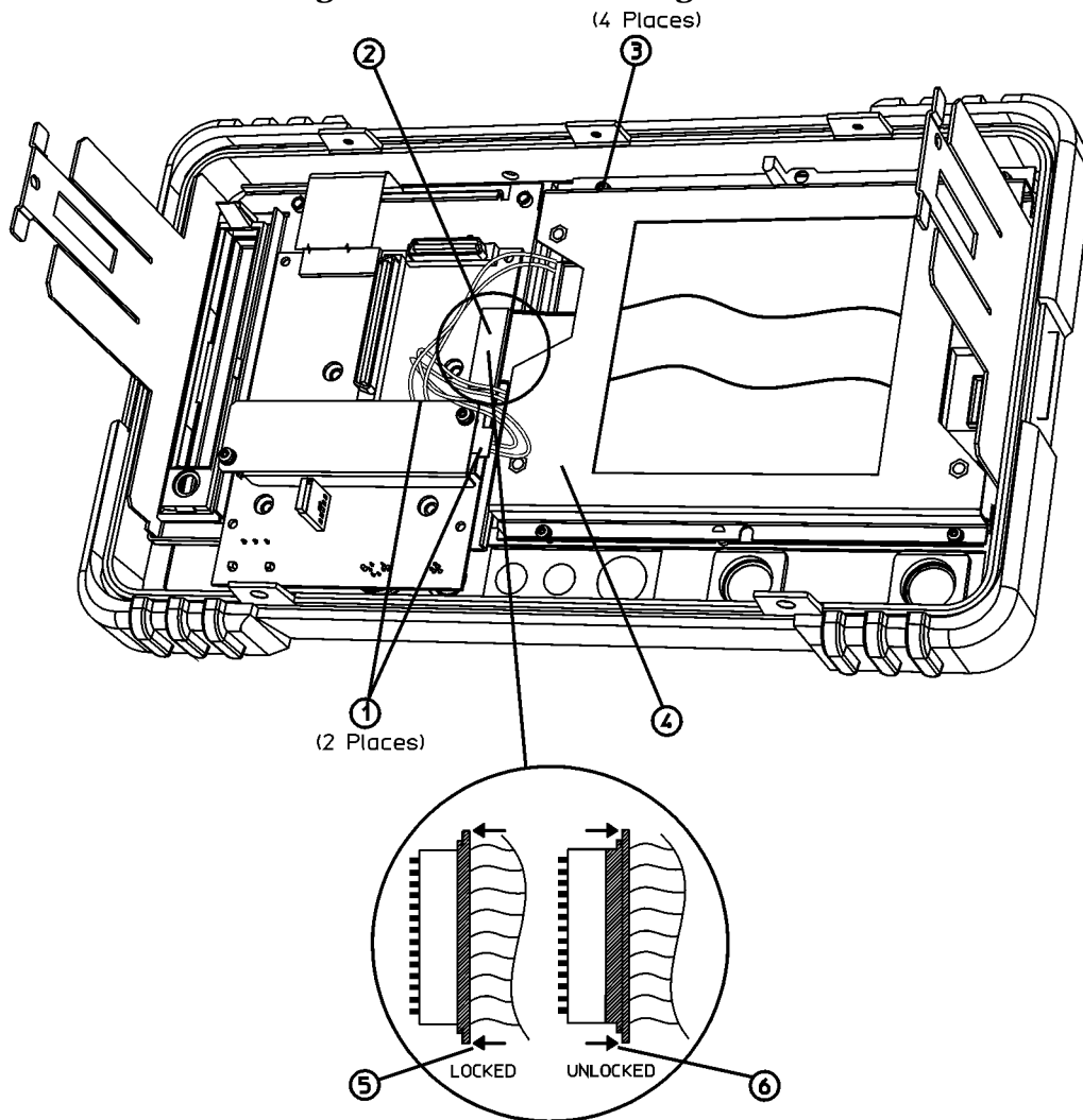
Figure 6 Disconnecting the Front Frame Wiring Connections
