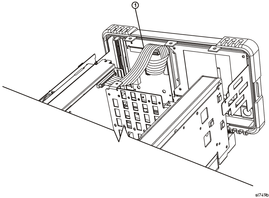
Figure 16 Front Frame Ribbon Cable
